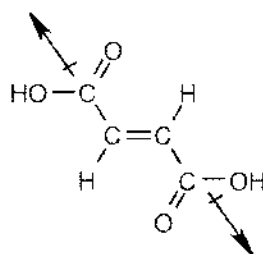
Fumaric acid
