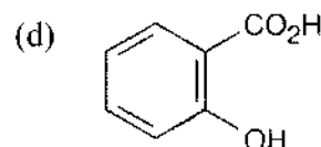
o -Hydroxybenzoic acid
