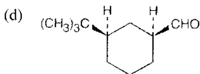
cis -3- tert -Butylcyclohexanecarbaldehyde
