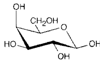
\beta -D-Galactopyranose [\alpha]_D = +52.8^\circ
