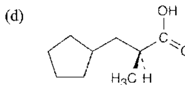
( S )-3-Cyclopentyl-2-methylpropanoic acid
