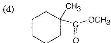
Methyl 1-methylcyclohexanecarboxylate
