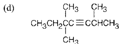
2,5,5-Trimethyl-3-heptyne
