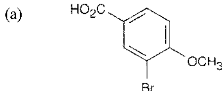
3-Bromo-4-methoxybenzoic acid
