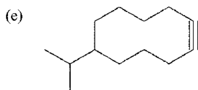
6-Isopropylcycloodecyne
