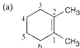
1,2-Dimethylcyclohexene
