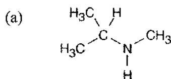
N -Methylisopropylamine
