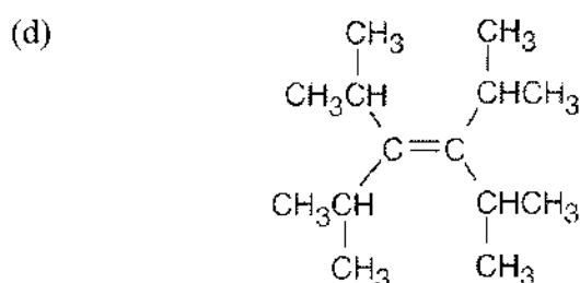
3,4-Diisopropyl-2,5-dimethyl-3-hexene
