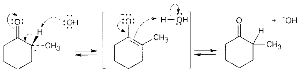
(R) -2-Methylcyclohexanone
