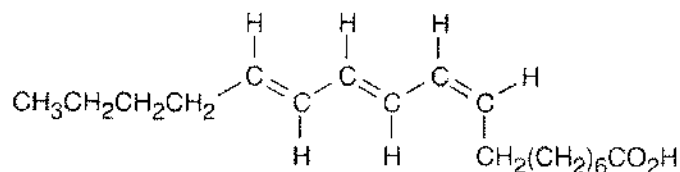
(9 Z ,11 E ,13 E )-9,11,13-Octadecatrienoic acid (Eleostearic acid)
