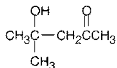
4-Hydroxy-4-methyl-2-pentanone
