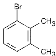
1-Bromo-2,3-dimethylbenzene
