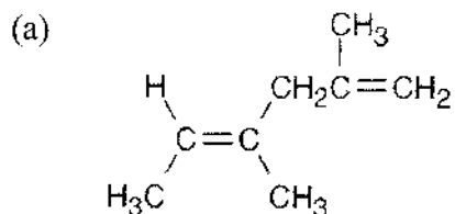
(4E)-2,4-Dimethyl-1,4-hexadiene
