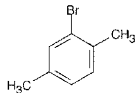
2-Bromo-1,4-dimethylbenzene
