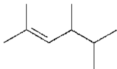
2,4,5-Trimethyl-2-hexene
