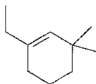
1-Ethyl-3,3-dimethylcyclohexene
