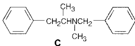
Benzphetamine (an appetite suppressant)
