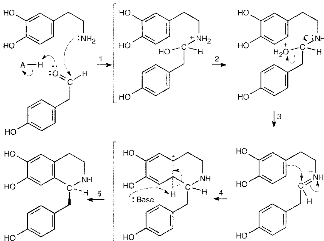
(S)-Norcoclaurine
