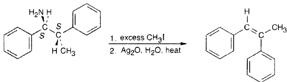
(1 S ,2 S )-(1,2-Diphenylpropyl)amine
