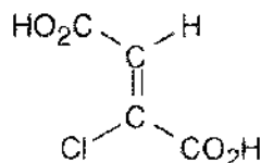
(Z)-2-Chloro-2-butene-1,4-dioic acid
