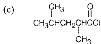
2,4-Dimethylpentanoyl chloride
