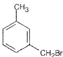
m -(Bromomethyl)toluene
