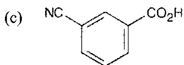
m -Cyanobenzoic acid
