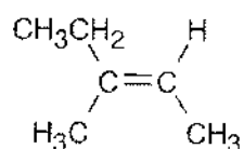
(E)-3-Methyl-2-pentene
