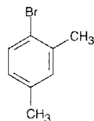
1-Bromo-2,4-dimethylbenzene
