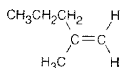
2-Methyl-1-pentene
