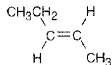
( E )-2-Pentene
