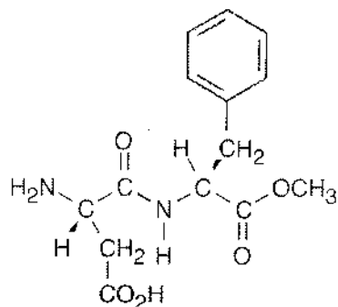
Aspartame (nonzwitterionic form)
