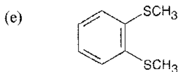
o -(Dimethylthio)benzene
