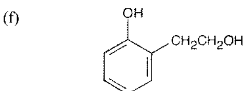
o -(2-Hydroxyethyl)phenol
