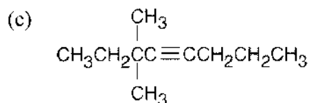
3,3-Dimethyl-4-octyne
