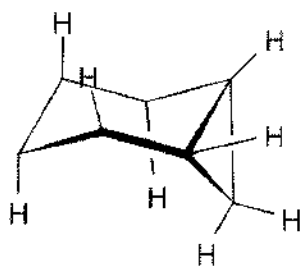
cis -Bicyclo[4.1.0]heptane
