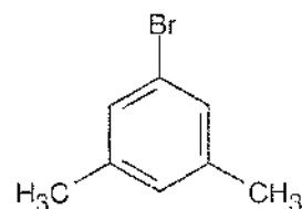
1-Bromo-3,5-dimethylbenzene
