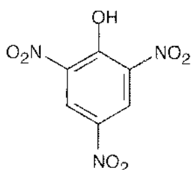
2,4,6-Trinitrophenol
