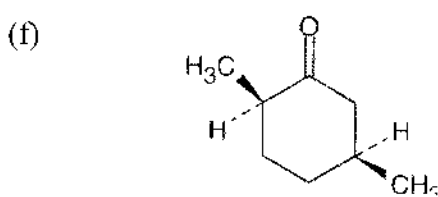
cis -2,5-Dimethylcyclohexanone
