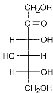
D-Sorbose
