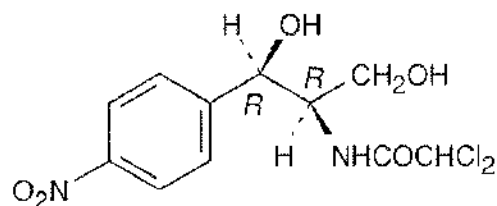
Chloramphenicol
