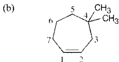
4,4-Dimethylcycloheptene
