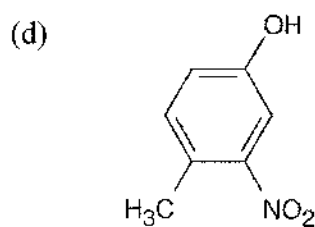
4-Methyl-3-nitrophenol
