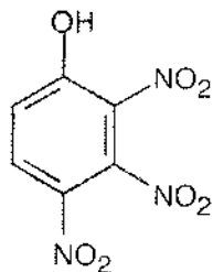
2,3,4-Trinitrophenol
