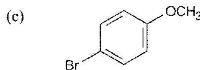
p -Bromoanisole
