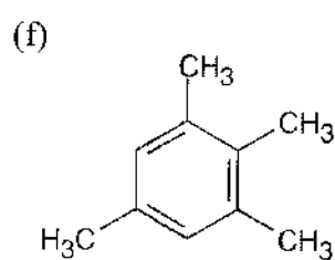
1,2,3,5-Tetramethylbenzene
