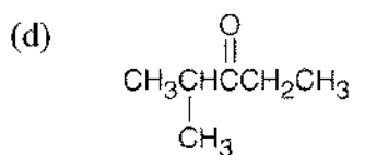
2-Methyl-3-pentanone
