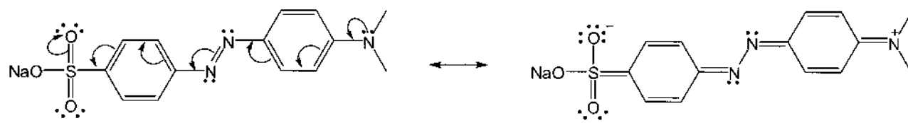
Methyl Orange
