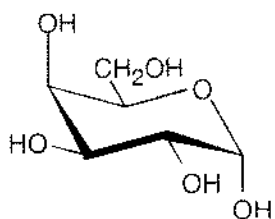
\alpha -D-Galactopyranose [\alpha]_D = +150.7^\circ
