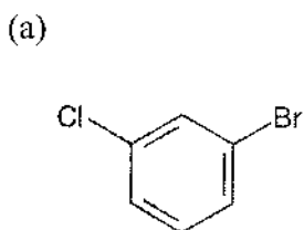
m -Bromochlorobenzene
