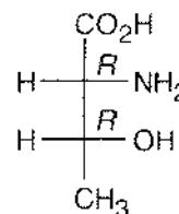
Diastereomers of Threonine
