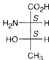
Diastereomers of Threonine
