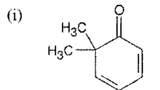
6,6-Dimethyl-2,4-cyclohexadienone
