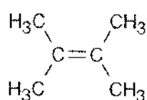
2,3-Dimethyl-2-butene
