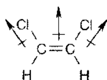
cis -1,2-Dichloroethylene
