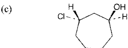
trans -3-Chlorocycloheptanol and enantiomer
