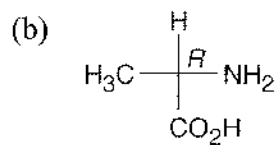
(R)-Alanine CH 3 CH(NH 2 )CO 2 H
