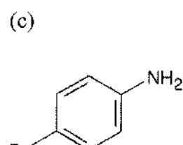
p -Bromoaniline
