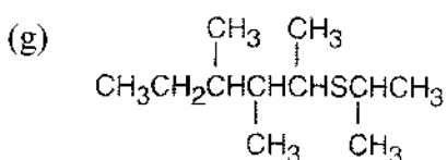
2-(Isopropylthio)-3,4- dimethylhexane
