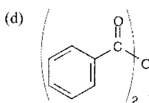
Benzoic anhydride
