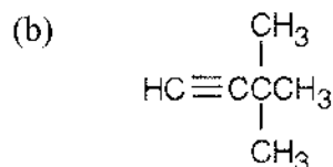
3,3-Dimethyl-1-butyne
