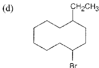
1-Bromo-4-ethylcyclodecane
