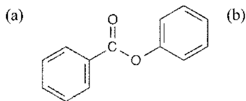
Phenyl benzoate
