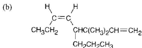
cis -3,3-Dimethyl-4-propyl-1,5-octadiene
