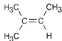
2-Methyl-2-butene
