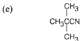
2,2-Dimethylpropanenitrile
