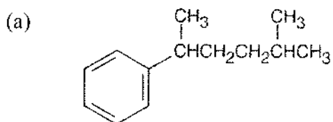
2-Methyl-5-phenylhexane
