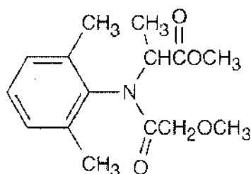
C Metalaxyl (a fungicide)
