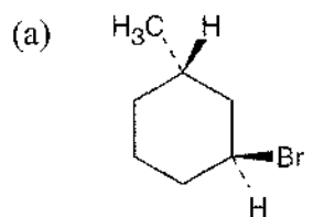
trans -1-Bromo-3-methylcyclohexane
