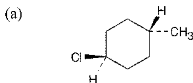
trans -1-Chloro-4-methylcyclohexane
