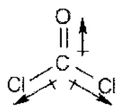
Phosgene
