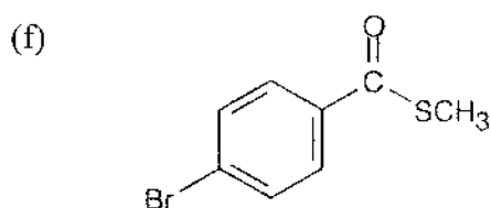
Methyl p -bromobenzenethioate
