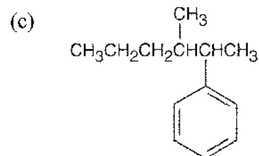
3-Methyl-2-phenylhexane
