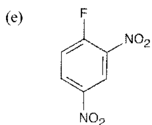
1-Fluoro-2,4-dinitrobenzene
