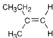
2-Methyl-1-butene
