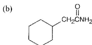
Cyclohexylacetamide
