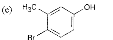
4-Bromo-3-methylphenol
