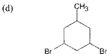
1,3-Dibromo-5-methylcyclohexane
