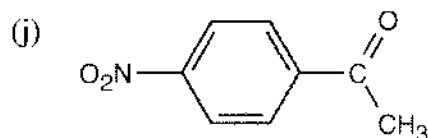
p -Nitroacetophenone
