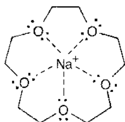
15-Crown-5
