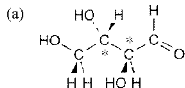
Threose
