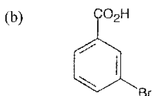
m -Bromobenzoic acid
