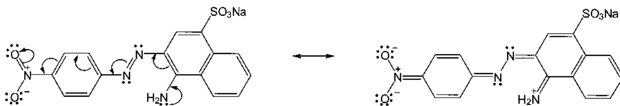
C.I. Acid Red 74
