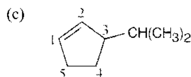
3-Isopropylcyclopentene
