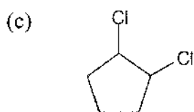
1,2-Dichlorocyclopentane
