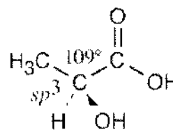
Lactic acid
