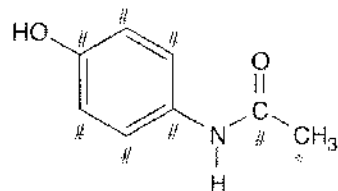
Acetaminophen
