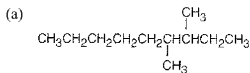
3,4-Dimethylnonane
