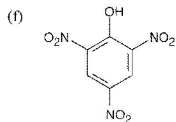
2,4,6-Trinitrophenol
