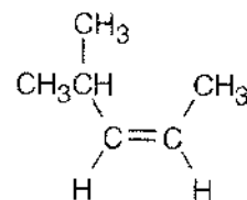
(Z)-4-Methyl-2-pentene
