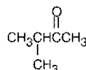
3-Methyl-2-butanone
