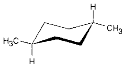
trans -1,4-Dimethylcyclohexane
