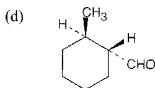
trans -2-Methylcyclohexanecarbaldehyde
