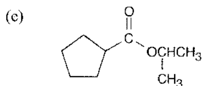
Isopropyl cyclopentanecarboxylate
