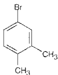
4-Bromo-1,2-dimethylbenzene
