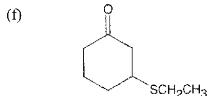
3-(Ethylthio)cyclohexanone
