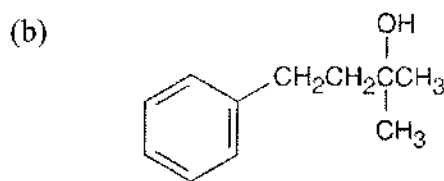
2-Methyl-4-phenyl-2-butanol
