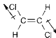
trans -1,2-Dichloroethylene
