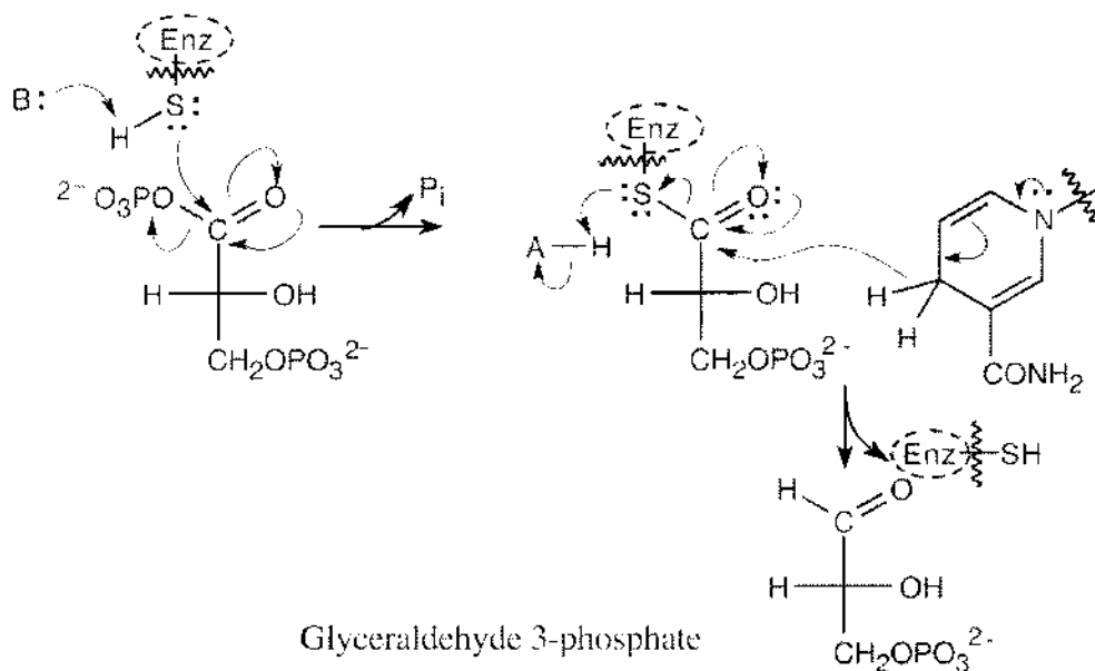
Glyceraldehyde 3-phosphate
