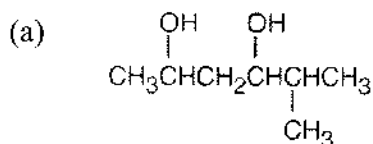
5-Methyl-2,4-hexanediol
