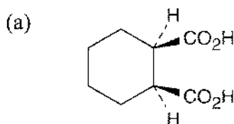
cis -1,2-Cyclohexanedicarboxylic acid
