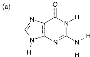
Guanine (G) DNA RNA
