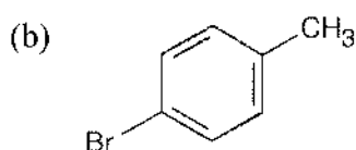
p -Bromotoluene
