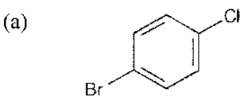
p -Bromochlorobenzene
