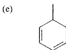
5-Methyl-1,3-cyclohexadiene
