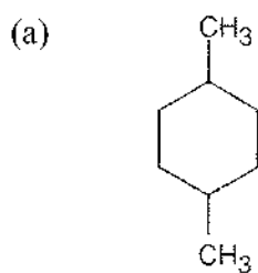
1,4-Dimethylcyclohexane
