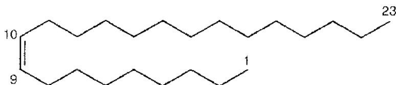
cis -9-Tricosene
