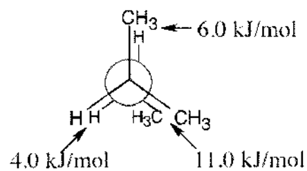
Least stable conformation
