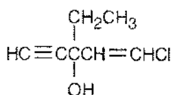
Ethchlorvynol (a sedative)
