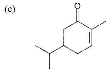
5-Isopropyl-2-methyl-2-cyclohexenone
