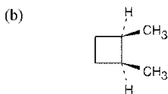
cis -1,2-Dimethylcyclobutane
