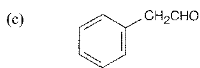
Phenylacetaldehyde
