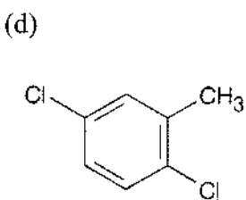
2,5-Dichlorotoluene
