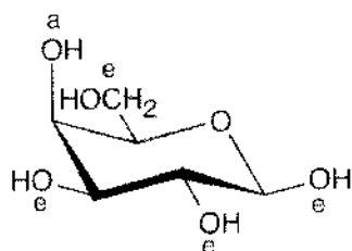
\beta -D-Galactopyranose
