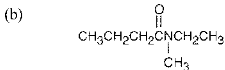
N -Ethyl- N -methylbutanamide
