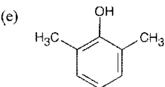
2,6-Dimethylphenol
