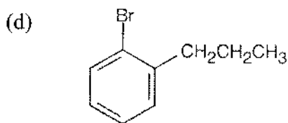
o -Bromopropylbenzene
