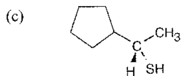
(S) -1-Cyclopentylethanethiol
