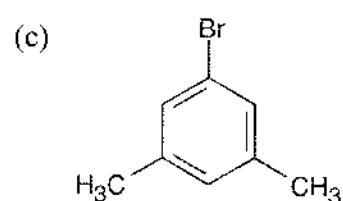
1-Bromo-3,5-dimethylbenzene
