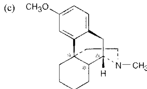
Dextromethorphan
