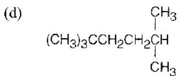
2,2,5-Trimethylhexane
