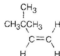
3,3-Dimethyl-1-butene
