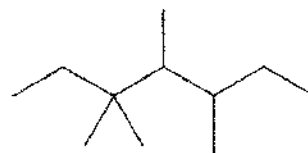
3,3,4,5-Tetramethylheptane
