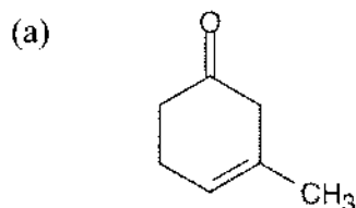
3-Methyl-3-cyclohexenone
