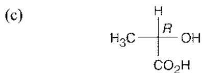
(R)-2-Hydroxypropanoic acid CH 3 CH(OH)CO 2 H
