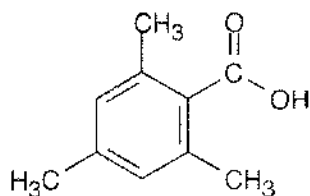
2,4,6-Trimethylbenzoic acid
