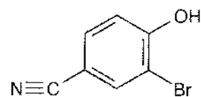
2-Bromo-4-cyanophenol
