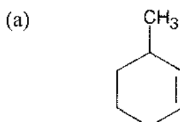
3-Methylcyclohexene
