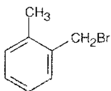
o -(Bromomethyl)toluene
