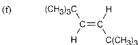
trans -2,2,5,5-Tetramethyl-3-hexene
