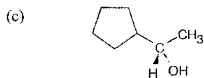
(S)-1-Cyclopentylethanol
