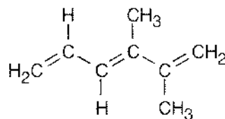
2,3-Dimethyl-1,3,5-hexatriene
