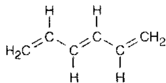
1,3,5-Hexatriene
