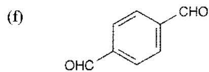
p -Benzenedicarbaldehyde
