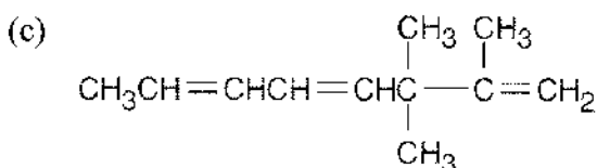
2,3,3-Trimethyl-1,4,6-octatriene
