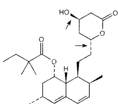
Simvastatin (Zocor)
