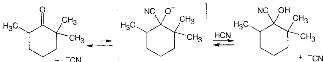
2,2,6-Trimethylcyclohexanone
