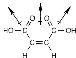
Maleic acid
