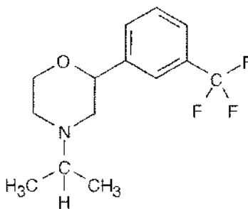
B Oxaflozane (an antidepressant)
