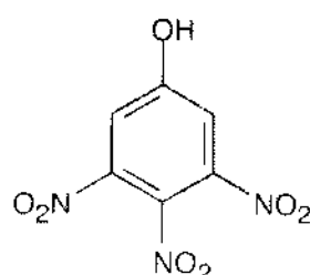
3,4,5-Trinitrophenol
