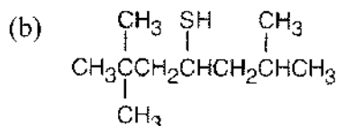
2,2,6-Trimethyl-4-heptanethiol
