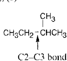
2-Methylbutane
