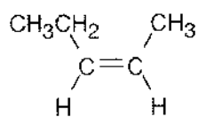
( Z )-2-Pentene
