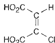
(E)-2-Chloro-2-butene-1,4-dioic acid
