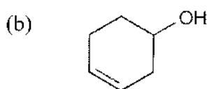
3-Cyclohexen-1-ol
