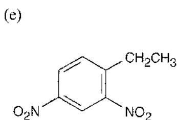
1-Ethyl-2,4-dinitrobenzene
