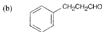
3-Phenylpropanal
