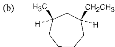
cis -1-Ethyl-3-methylcycloheptane
