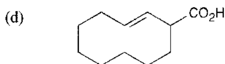
(E) -2-Cyclodecenecarboxylic acid
