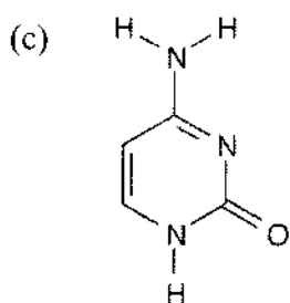
Cytosine (C) DNA RNA
