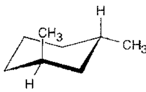
trans -1,3-Dimethylcyclohexane
