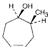
cis -2-Methyl-4-cyclohepten-1-ol
