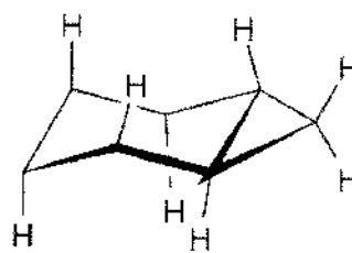
trans -Bicyclo[4.1.0]heptane
