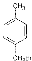
p -(Bromomethyl)toluene
