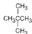
2,2-Dimethylpropane
