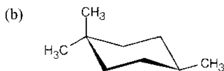
1,1,4-Trimethylcyclohexane
