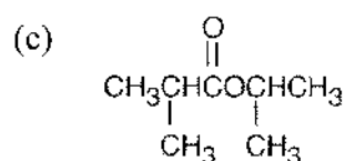
Isopropyl 2-methylpropanoate
