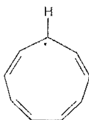
radical 9 \pi electrons
