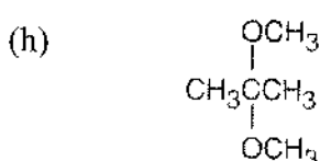
2,2-Dimethoxypropane
