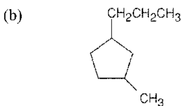
1-Methyl-3-propylcyclopentane
