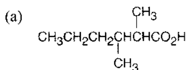
2,3-Dimethylhexanoic acid
