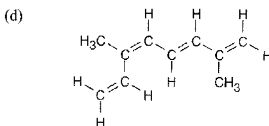
(3E,5Z)-2,6-Dimethyl-1,3,5,7-octatetraene
