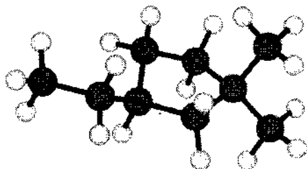
3-Ethyl-1,1-dimethylcyclopentane
