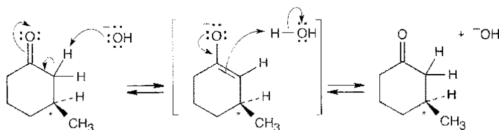
(S) -3-Methylcyclohexanone
