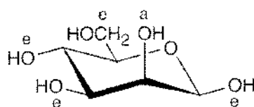
\beta -D-Mannopyranose
