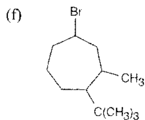
4-Bromo-1- tert -butyl-2-methylcycloheptane
