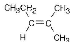
2-Methyl-2-pentene
