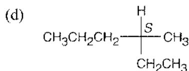
(S)-3-Methylhexane CH 3 CH 2 CH 2 CH(CH 3 )CH 2 CH 3
