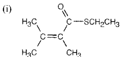
Ethyl 2,3-dimethyl- 2-butenethioate
