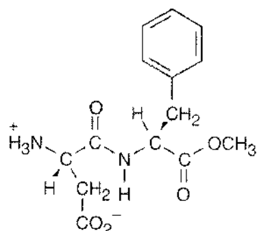
Aspartame at pH = 5.9, 7.3
