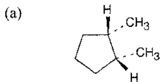
cis -1,2-Dimethylcyclopentane
