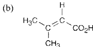
3-Methyl-2-butenoic acid
