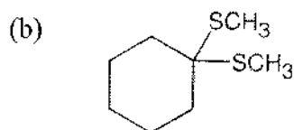
1,1-(Dimethylthio)- cyclohexane
