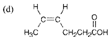
(Z)-4-Hexenoic acid
