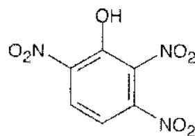
2,3,6-Trinitrophenol
