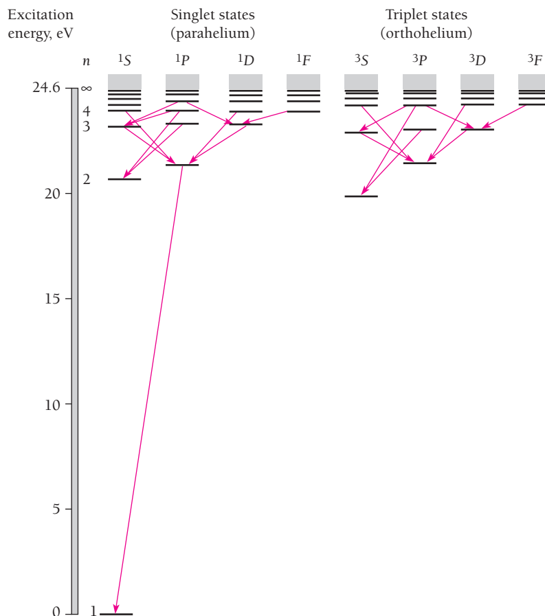
Figure 7.24 Energy-level diagram for helium showing the division into singlet (parahelium) and triplet (orthohelium) states. There is no 1^3S state because the exclusion principle prohibits two electrons with parallel spins in the same state.
