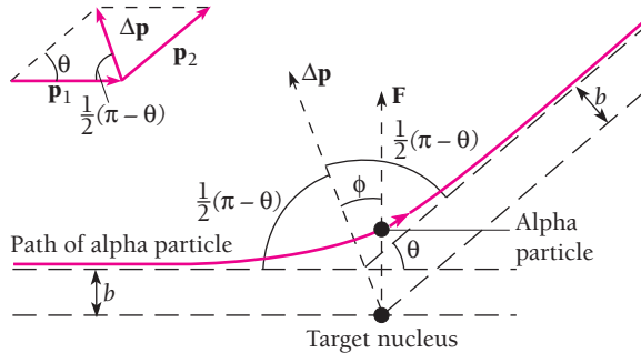
Figure 4.31 Geometrical relationships in Rutherford scattering.
