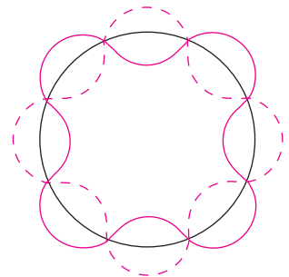
Circumference = 4 wavelengths
