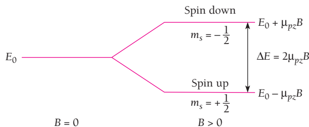
Figure 11.5 The energy levels of a proton in a magnetic field are split into spin-up ( S_z parallel to \mathbf{B} ) and spin-down ( S_z antiparallel to \mathbf{B} ) sublevels.
