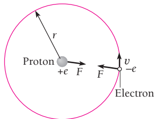
Figure 4.5 Force balance in the hydrogen atom.
