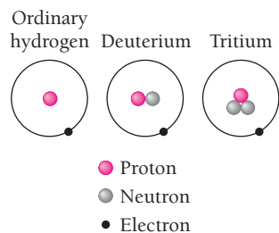
Figure 11.1 The isotopes of hydrogen.
