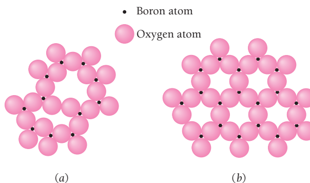
Figure 10.1 Two-dimensional representation of \text{B}_2\text{O}_3 . (a) Amorphous \text{B}_2\text{O}_3 exhibits only short-range order. (b) Crystalline \text{B}_2\text{O}_3 exhibits long-range order as well.
