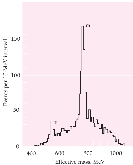
Figure 13.4 Resonant states in the reaction \pi^+ + p \rightarrow \pi^+ + p + \pi^+ + \pi^- + \pi^0 occur at effective masses of 549 and 783 MeV/ c^2 . By effective mass is meant the total energy, including mass energy, of the three new mesons relative to their center of mass.
