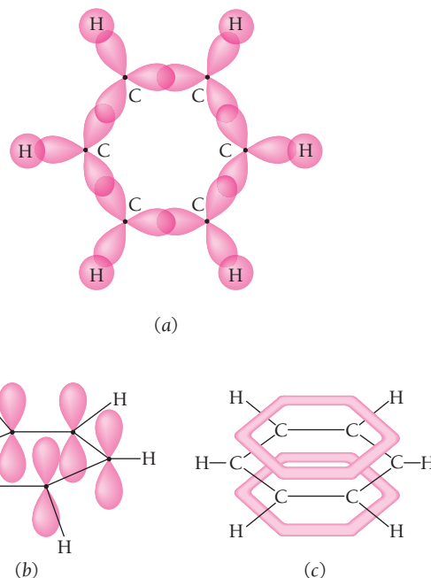
Figure 8.15 The benzene molecule. (a) The overlaps between the sp^2 hybrid orbitals in the C atoms with each other and with the s orbitals of the H atoms lead to \sigma bonds. (b) Each C atom has a pure p_x orbital occupied by one electron. (c) The bonding \pi molecular orbitals formed by the six p_x atomic orbitals constitute a continuous electron probability distribution around the molecule that contains six delocalized electrons.
