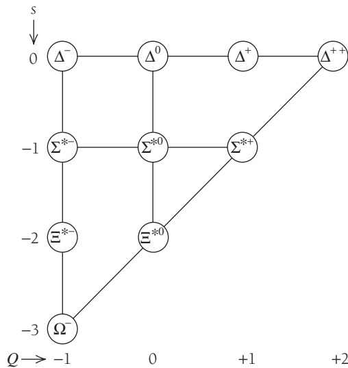
Figure 13.7 Baryon supermultiplet whose members have spin \frac{3}{2} and (except \Omega^- ), are short-lived resonance particles. The \Xi^{*-} and \Sigma^{*-} particles here are heavier and have different spins from the ones in Table 13.3. The \Omega^- particle was predicted from this scheme.
