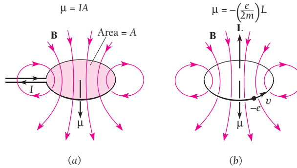
Figure 6.16 (a) Magnetic moment of a current loop enclosing area A . (b) Magnetic moment of an orbiting electron of angular momentum \mathbf{L} .
