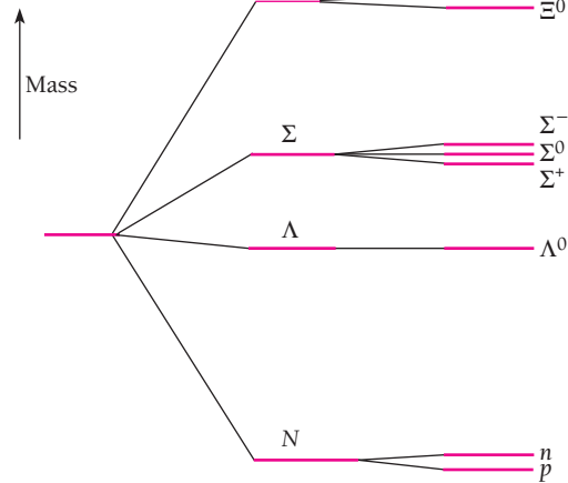
Figure 13.8 Origin of the baryon supermultiplet shown in Fig. 13.5.
